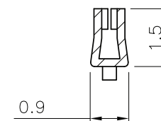
C-C SEC
