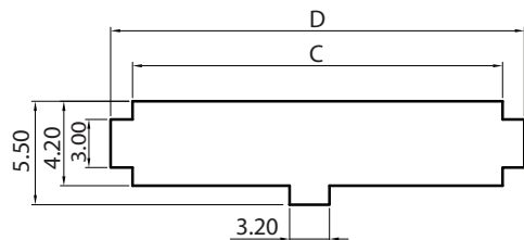
RECOMMENDED PANEL COUTOUT
