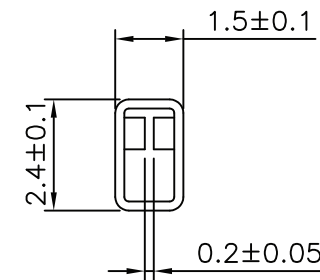
C-C SEC
