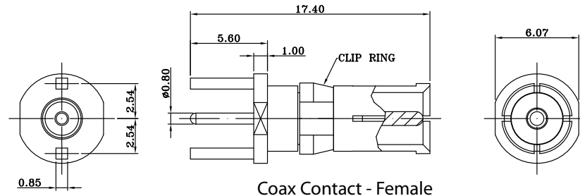
Coax Contact - Female
