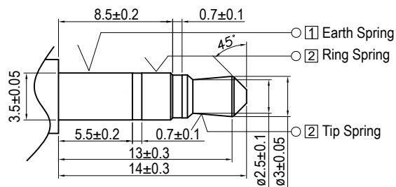
RECOMMENDED MATING PLUG
