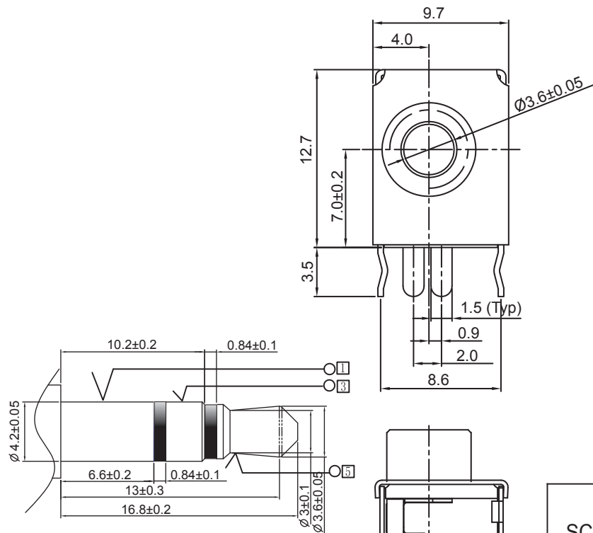
RECOMMENDED MATING PLUG
