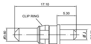
Power Contact - Male
