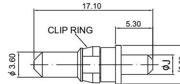
Power Contact - Male
