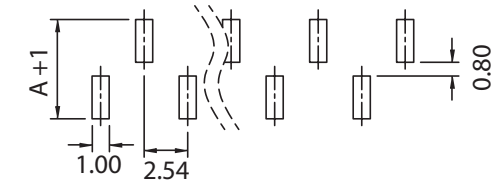
RECOMMENDED PCB LAYOUT TYPE B
