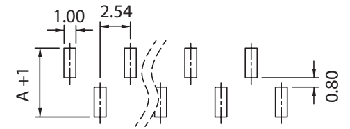
RECOMMENDED PCB LAYOUT TYPE A
