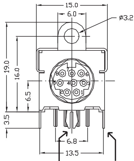
TERMINAL TAB (1)
