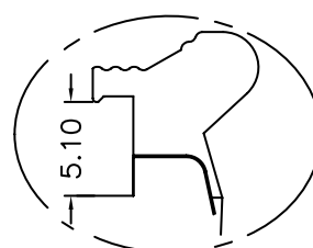
Short Ejector Latch
