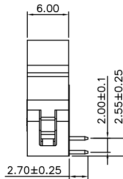
Short Ejector Latch
