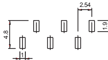
FOOTPRINT TYPE 2
