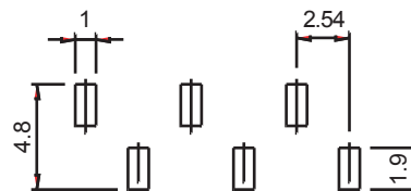
FOOTPRINT TYPE 1
