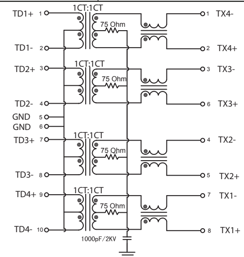
SCHEMATIC DIAGRAM
